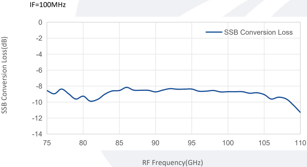
SSB Covernion Loss vs RF Frequency
