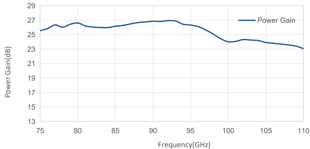
Power Gain vs Frequency
